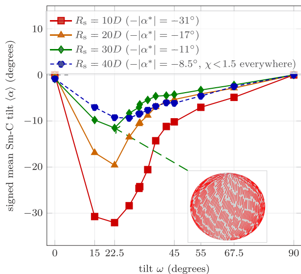
FIG. 4. Signed mean Sm-C tilt \langle \alpha \rangle(\omega) vs \omega for the four host radii ( \ell = 5D ); the legend lists the P3 prediction -|\alpha^*| of Eq. (5) for each radius. The dashed horizontal line represents the Sm-A reference ( \alpha = 0 ); the R_s = 40D trace is indicated by the dashed line. The magnitude divided by the per-host width \sigma_\alpha gives the chirality index of Fig. 5. Inset (lower right): a representative coherent Sm-C texture [the (30, 8) host at \omega = 15^\circ , shown for the texture only; the traces are \ell = 5D ]; the long-dashed arrow marks the \omega = 22.5^\circ minimum of the R_s = 30D trace.
