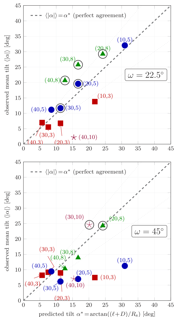
FIG. 3. Master test of the P3 tilt-angle formula [Eq. (5)]: observed mean layer tilt \langle |\alpha| \rangle vs the predicted \alpha^* = \arctan[(\ell + D)/R_s] for every (R_s, \ell) cohort for which the local smectic fit returns a defined mean tilt at the tilt slice shown, \omega = 22.5^\circ (top) and \omega = 45^\circ (bottom) (sparse panels whose fit does not converge are absent). The marker's shape and color encode rod length, and the dashed diagonal marks perfect prediction; the dotted lines mark \pm 25\% . The black rings single out the coherent Sm-C cohorts ( \chi \geq 1.5 with f_{sm} \geq 0.10 , classified in Fig. 6), the only points expected to lie on or near the diagonal. The unringed (10, 5) point at 22.5^\circ is a qualified case: single-handed and on the diagonal, but with layered patches too sparse to count as a coherent phase in Fig. 6. The remaining cohorts are Sm-A or multi-domain and are not expected to track the prediction. They are retained to show the negative controls rather than as positive evidence for the tilt scale. Near the origin, such points can fall close to the diagonal by coincidence: the unsigned mean of pure tilt noise is of order \sigma_\alpha = 6^\circ – 10^\circ , comparable with the small predicted values there.
