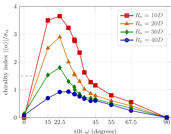
FIG. 5. Sm-C global chirality vs tilt \omega across host radii ( \ell = 5D ): the chirality index \chi = |\langle \alpha \rangle|/\sigma_\alpha for the same panels as Fig. 4. The horizontal dashed line marks the coherent-Sm-C threshold \chi = 1.5 : a host carries one coherent handedness at tilts where its curve lies above the line and is Sm-A or multi-domain where it lies below the line. The coherent-Sm-C label shown in Fig. 6 additionally requires f_{sm} \geq 0.10 . The dotted line marks \chi = 1 , the signed-tilt/noise scale used as a visual reference.
