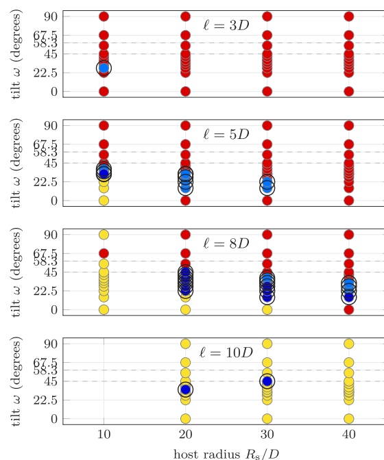
FIG. 6. Two-dimensional Sm-A/Sm-C phase diagrams on the (R_s, \omega) plane for \ell = 3D (top), 5D , 8D , and 10D (bottom). Each marker classifies one strict-MC panel by the smectic fraction and the chirality index: yellow bullet nematic ( f_{sm} < 0.10 ); red bullet Sm-A/noncoherent ( \chi < 1.5 ); light blue bullet coherent Sm-C with |\langle \alpha \rangle| \leq 22^\circ ; and dark blue bullet coherent Sm-C with |\langle \alpha \rangle| > 22^\circ (the 22^\circ bin edge is a display choice, not a physical threshold). The black rings mark the coherent Sm-C panels, the same marking as shown in Fig. 3. The nematic criterion takes precedence: a panel with a single-handed tilt but sparse layering, such as (10, 5) at low tilt, is classified nematic. The \ell = 10D panel has no R_s = 10D column: in that combination, the rod length equals the host radius ( \ell/R_s = 1 ) and it was not simulated.
