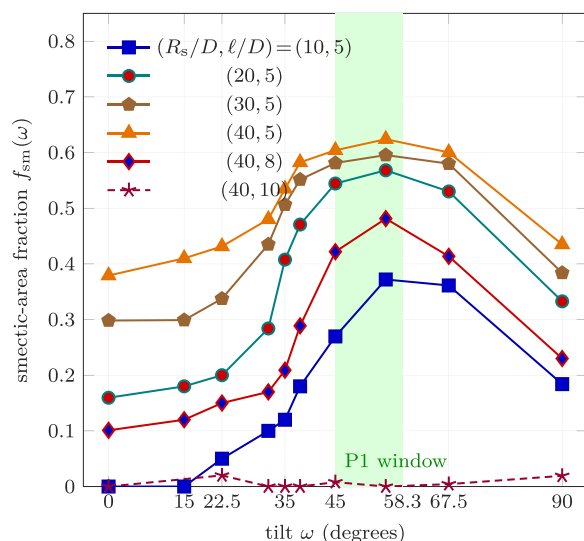
FIG. 2. Smectic-area fraction f_{sm}(\omega) across six (R_s, \ell) geometries (fraction of rods with a converged local fit and |\Psi^*| > 0.5 ). Shaded band: the smectic-area (P1) window [45^\circ, 58.3^\circ] [Eq. (3)]. The lower edge is the channel-swap symmetry point; the upper edge is the channel-saturation hypothesis and is not resolved separately by the present tilt grid. For clarity, only a subset of the tilt grid is shown; the \ell = 10D grid has no 15^\circ slice.
