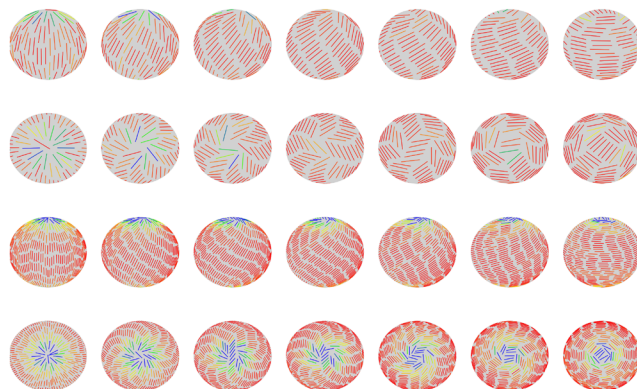
FIG. 1. Simulation snapshots at the locked tilts \omega = 0, 22.5^\circ, 35^\circ, 45^\circ, 55^\circ, 67.5^\circ , and 90^\circ (left to right) for two hosts. Top two rows: the smallest host R_s = 10D , \ell = 5D , side view (first row), and view along the polar axis (second row). Bottom two rows: the same but for the coherent-Sm-C host R_s = 20D and \ell = 5D . The rods are colored by their local nematic order parameter.
